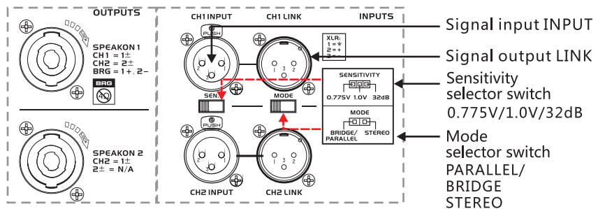
Signal connector
