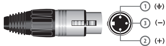
LINK Balanced connection base XLR
