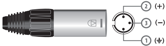
INPUT Balanced connection male XLR
